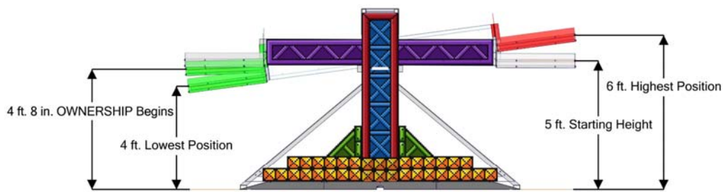
Figure 3-6: SCALE range of motion
