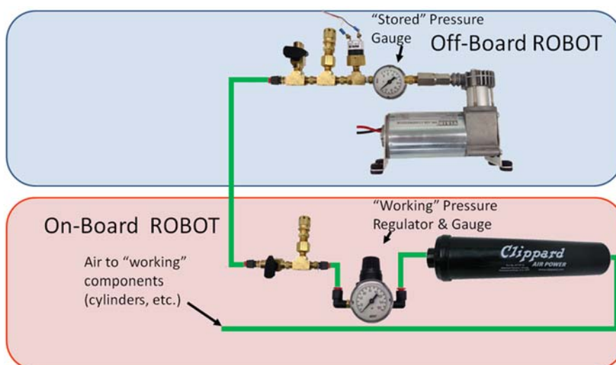
Figure 8-16: Off board compressor with stored pressure gauge and pressure switch off the ROBOT
